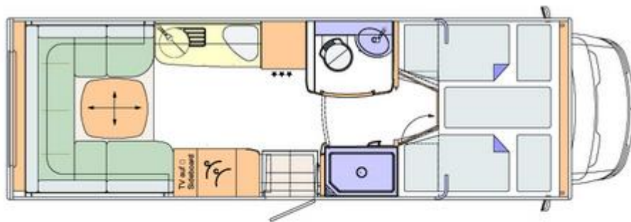
Cruiser Daily 791 RL
